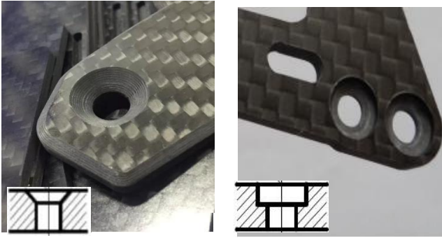
45 degree countersunk
